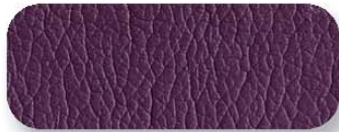
UL49 Port
